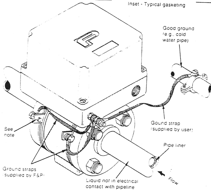
(B) Insulated pipe
