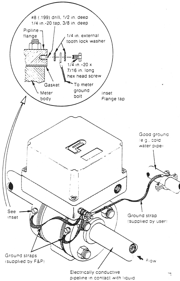
(A) Non-insulated pipe
